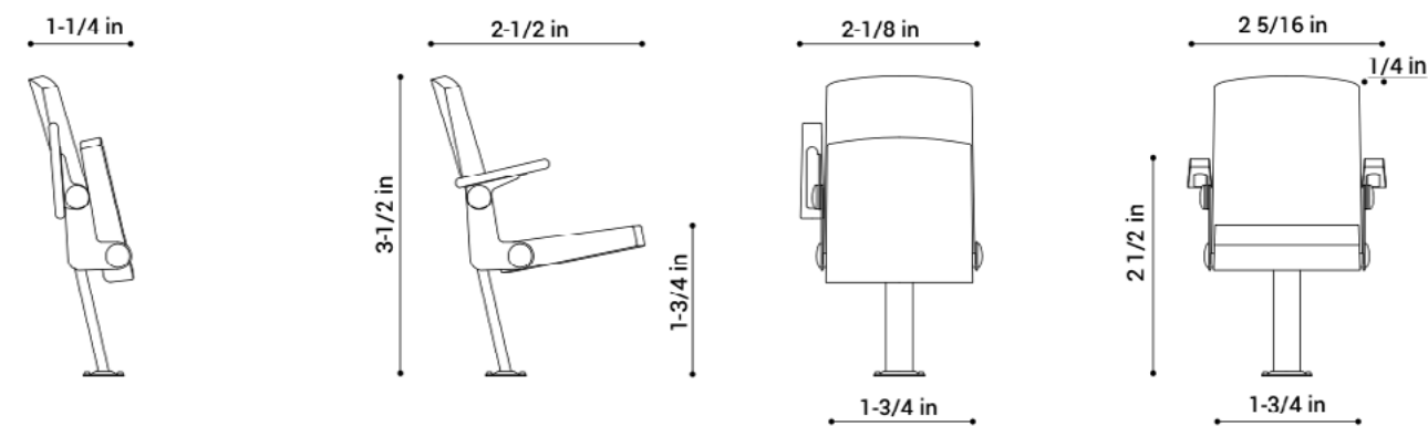
Foldable Armrests
