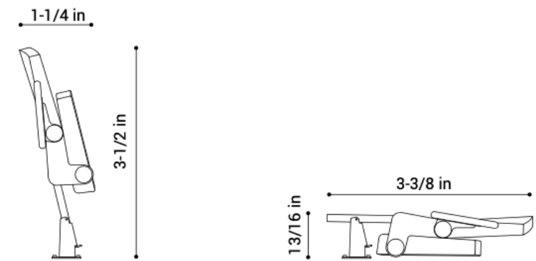
Foldable Armrests
